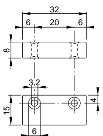
MG03 (Alnico in aluminium housing)
